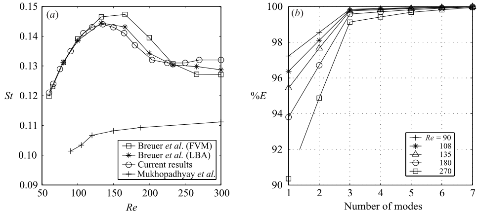
FIGURE 2. (a) Strouhal vs. Reynolds number ( \beta = 0.125 ). FVM: finite volume method; LBA: lattice-Boltzmann method. (b) Represented energy vs. mode number for different Reynolds numbers ( \beta = 0.125 ).
